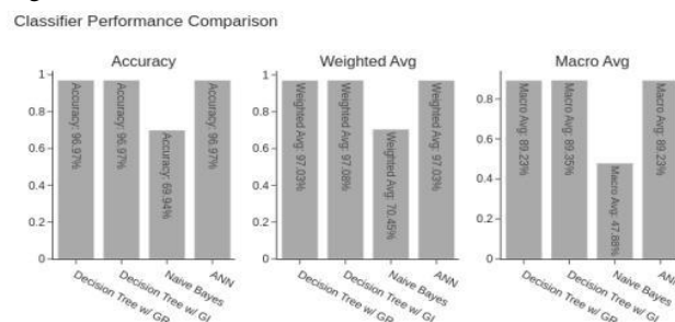
Fig. 3. Accuracy, weighted Average in which the weight is assigned as per the proportionality of the given value in the dataset, and Macro Average, in which the class imbalance problem is avoided as all the classes are treated with equal weightage.
