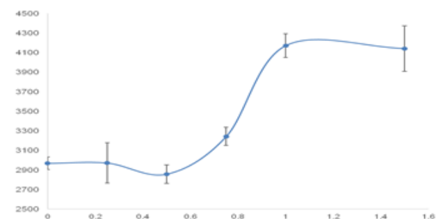
Figure 11: Suspension Consistency Vs Surface Roughness
