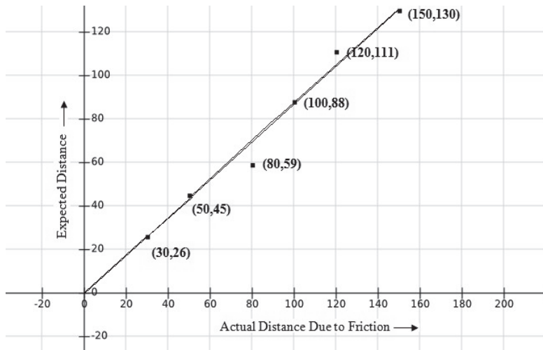
Figure 14: Expected vs Actual Distance Measure by Optical Encoders
