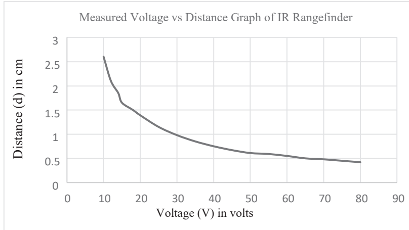
Figure 13: Measure Voltage vs. Distance Graph of IR Rangefinder
