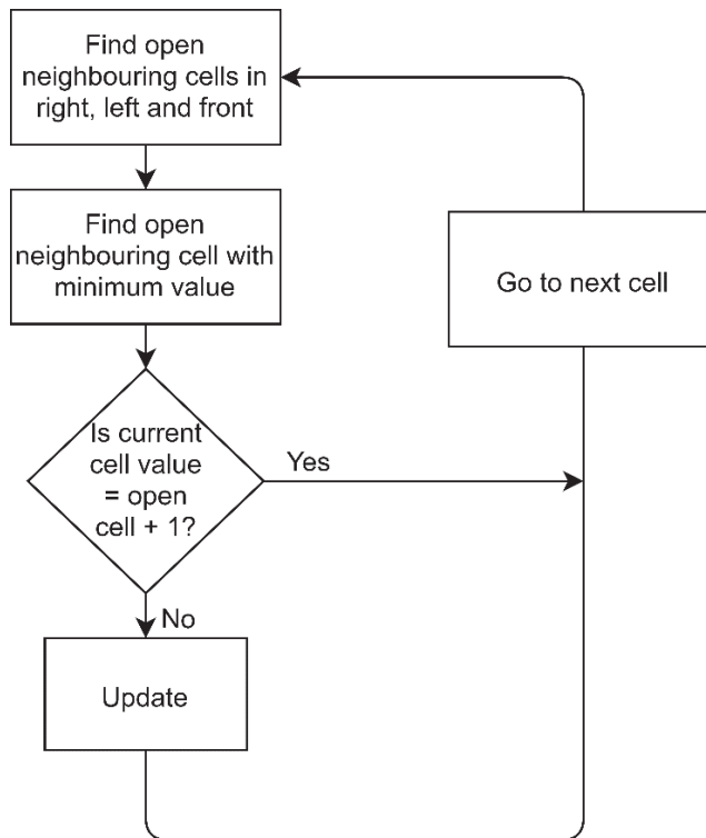
Figure 3: Floodfill algorithm
