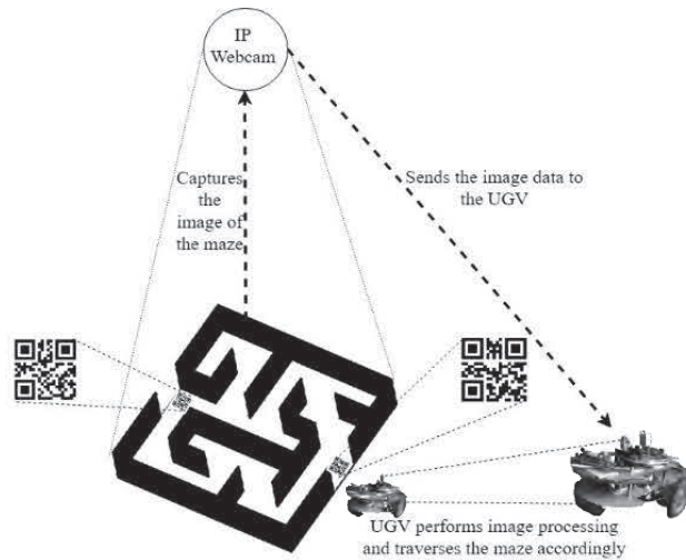
Figure 4: System Overview
