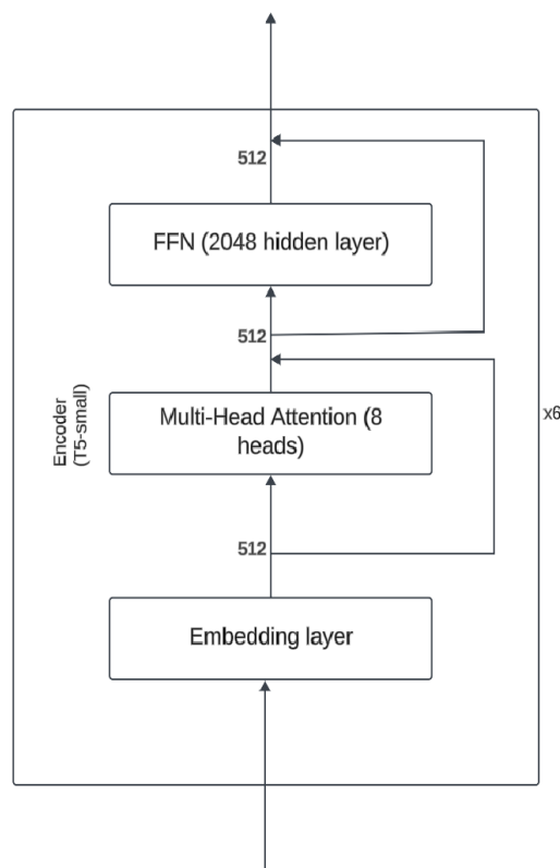
Figure 3. T5 Architecture
