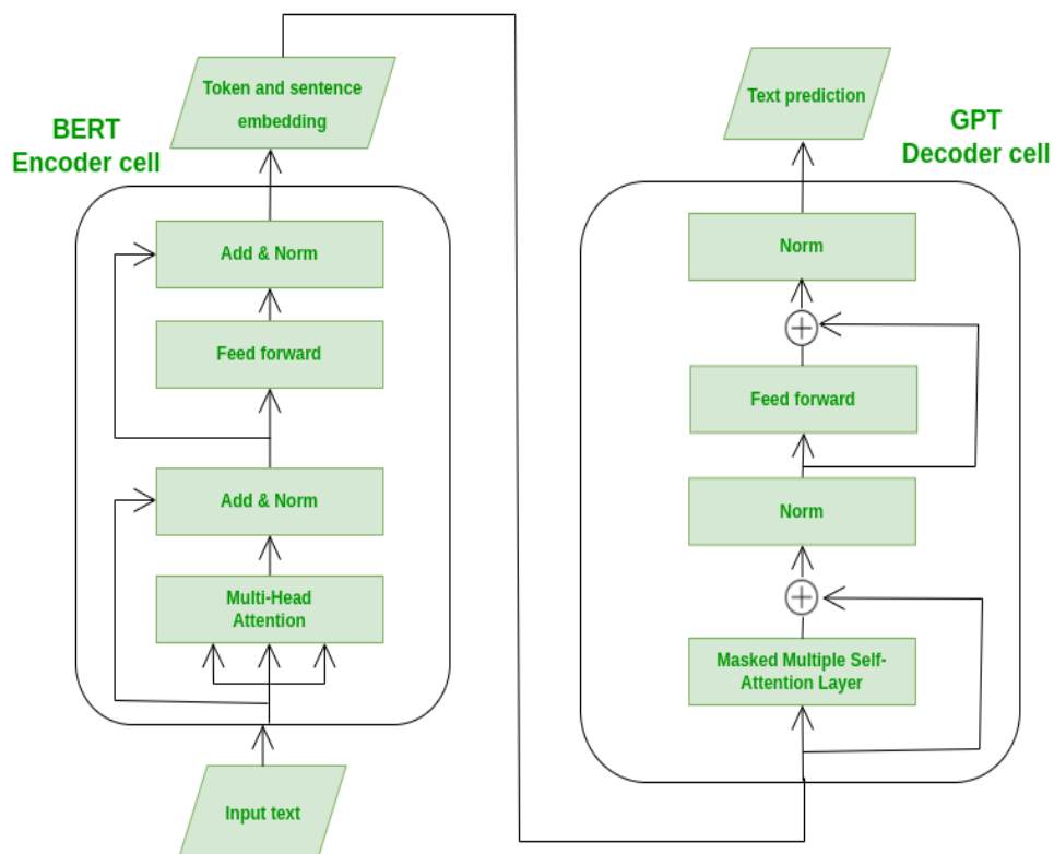
Figure 2. BART Architecture
