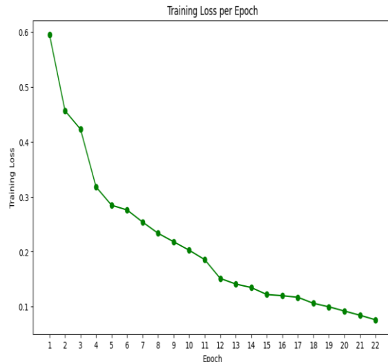
Figure 5. Training Loss per Epoch
