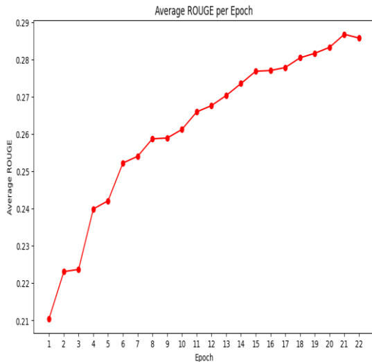
Figure 4. Average ROUGE per Epoch
