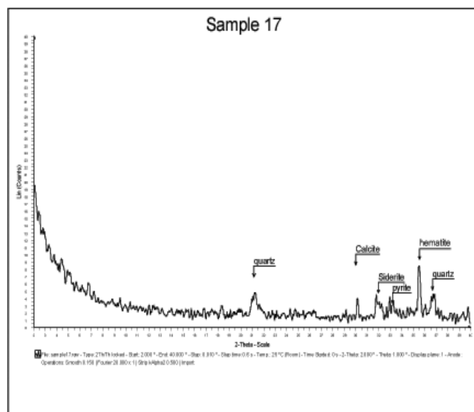
Fig. 7: X-ray Diffractogram of sample 17.
