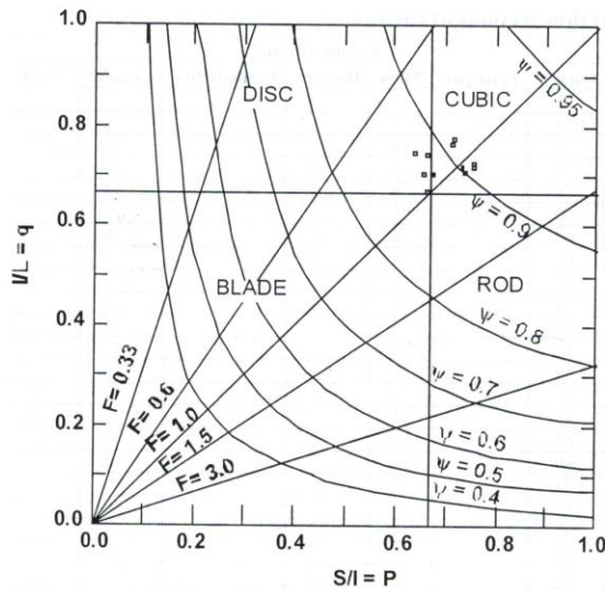
Fig. 5: Shape diagram indicating mean forms of aggregate samples
