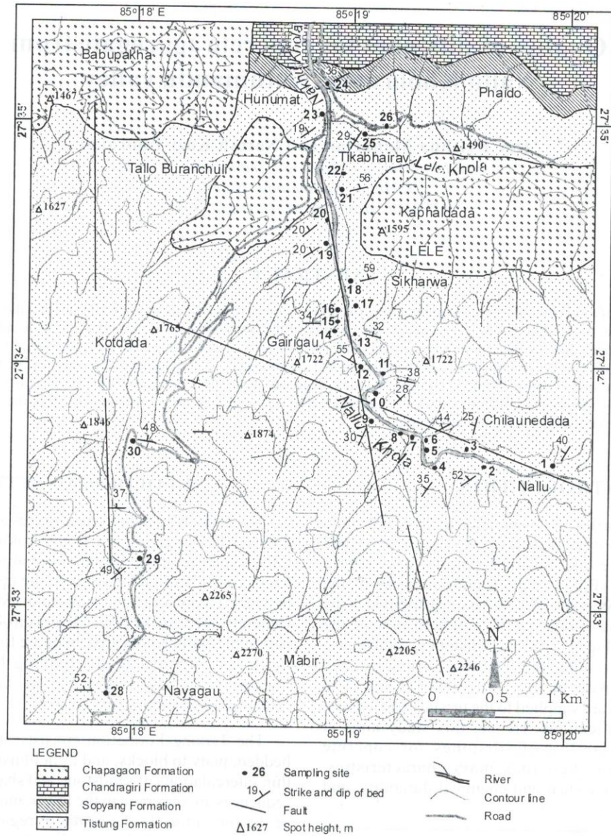
Fig. 2: Geological map with sampling sites (Geology: modified from Stöcklin and Bhattarai 1977)
