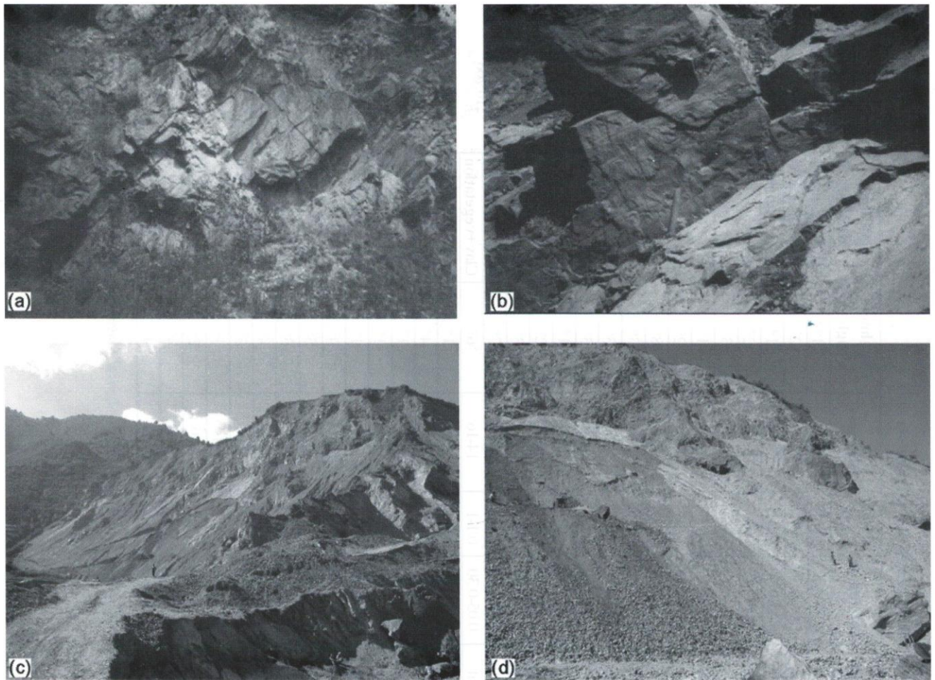
Fig. 3: Outcrops of rocks exposed in the banks and hill slopes of the Nallu Khola
