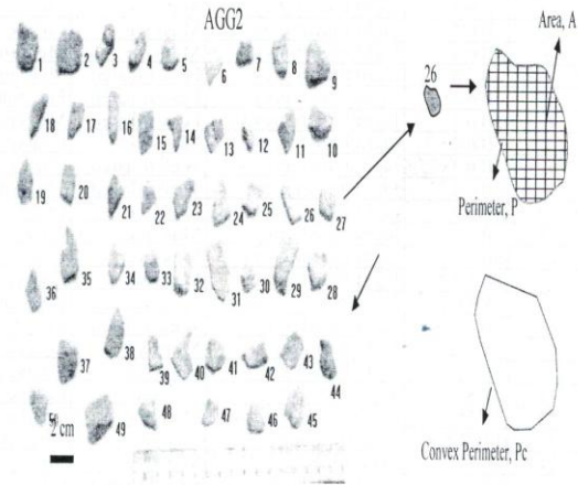
Fig. 6: Determination of perimeter and area of a grain. Sample 26 shown as an example.
