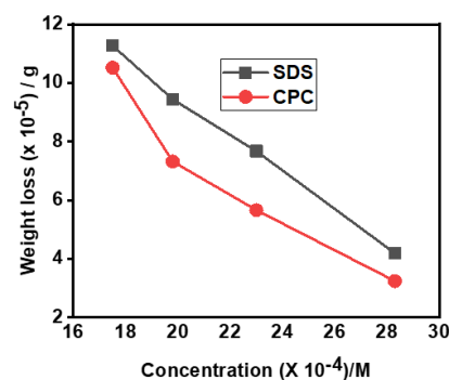
Figure 10: Representation of the variation of weight loss of mild steel of immersion time 3 hours in different concentrations
