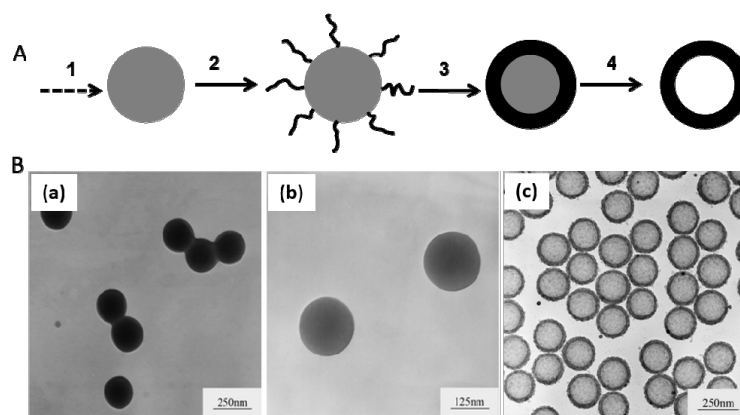
Figure 1. (A) Illustration of a conventional hard templating process for hollow sphere synthesis. Reprinted with permission from (9). (B) TEM pictures of (a) original PS particles, (b) PS/SiO 2 , and (c) hollow silica particles. Reprinted with permission from (10). Copyright 2007 American Chemical Society
