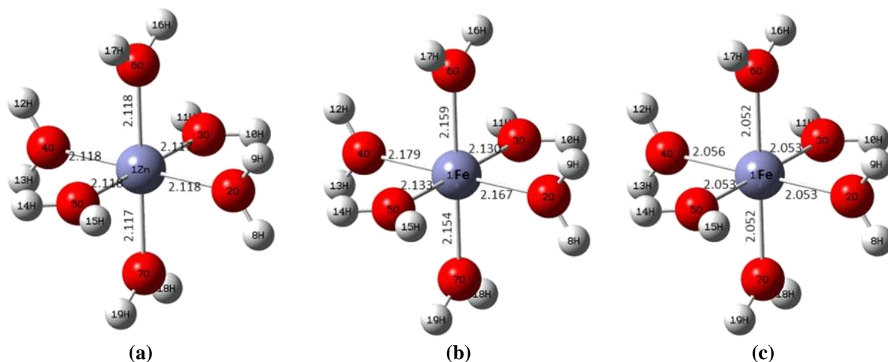
Fig. 2. The optimized structure of the complexes (a) [\text{Zn}(\text{H}_2\text{O})_6]^{2+} , (b) [\text{Fe}(\text{H}_2\text{O})_6]^{2+} , and (c) [\text{Fe}(\text{H}_2\text{O})_6]^{3+} .
