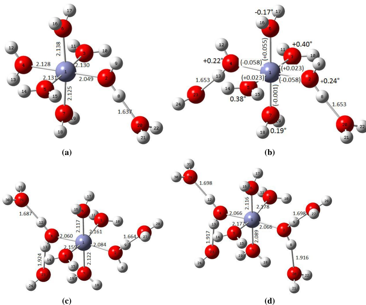
Fig. 3. The optimized structures of (a) [\text{Zn}(\text{H}_2\text{O})_6]^{2+}(\text{H}_2\text{O})_2^{2+} , (b) [\text{Zn}(\text{H}_2\text{O})_6]^{2+}(\text{H}_2\text{O})_2^{2+} , (c) [\text{Zn}(\text{H}_2\text{O})_6]^{2+}(\text{H}_2\text{O})_3^{2+} , and (d) [\text{Zn}(\text{H}_2\text{O})_6]^{2+}(\text{H}_2\text{O})_4^{2+} . In (b) changes in bond length are shown.
