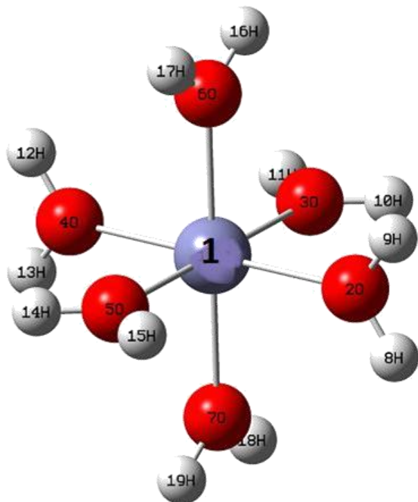
Fig.1. Structure of a metal complex with coordination number 6. The metal ion is at the center and water molecules are around it.
