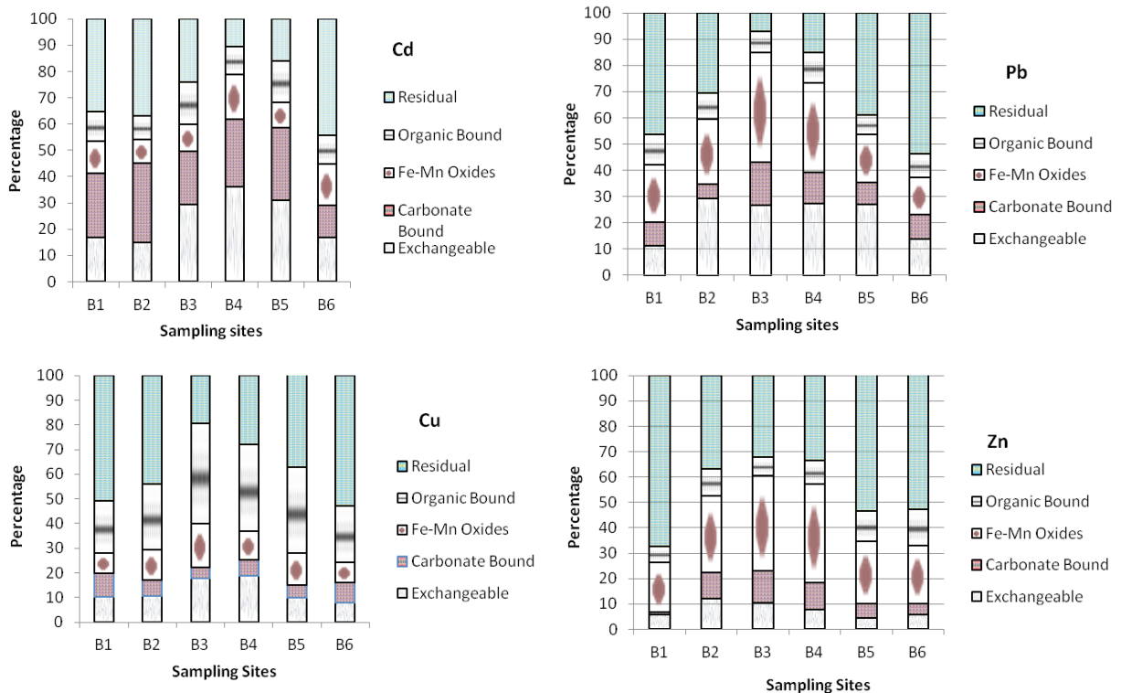
Figure 2 : Metal fraction in sediments of the Bagmati River (Exchangeable, carbonate, Fe-Mn oxide, organic and residual)
