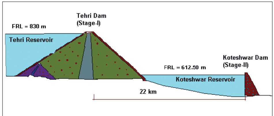
Figure 2. Sketch of Tehri and Koteshwar Dams
